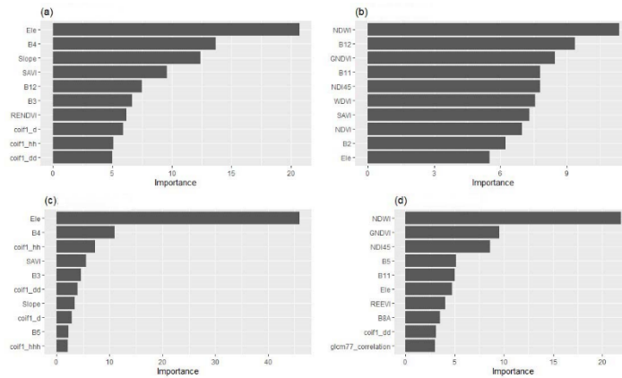
Figure 3. The importance ranking of the top 10 variables identified by (a) evergreen RF model; (b) deciduous RF model; (c) evergreen SGB model; and (d) deciduous SGB model
