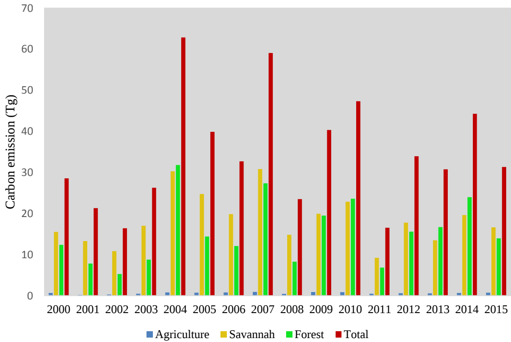
Figure 4. Annual Carbon Emissions from Vegetation Fires in Myanmar (2000-2015) Source: Based on data from GFED4s [9]
