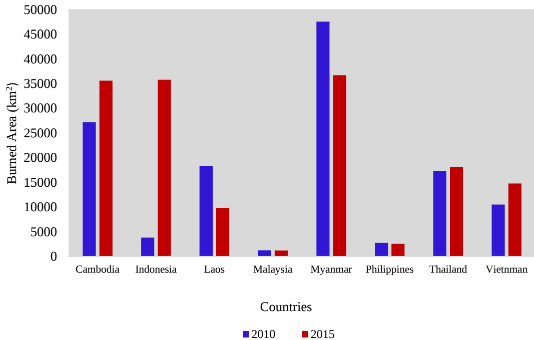
Figure 5. Burned Areas in SEA Countries (2010-2015)
