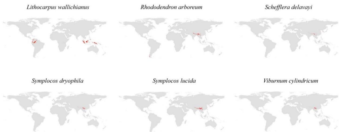
Figure 6. Suitable habitat ranges of upward category species.
