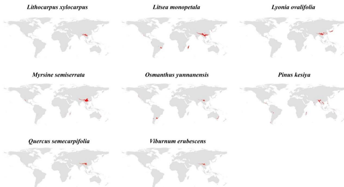
Figure 7. Suitable habitat ranges of non-upward category species.
