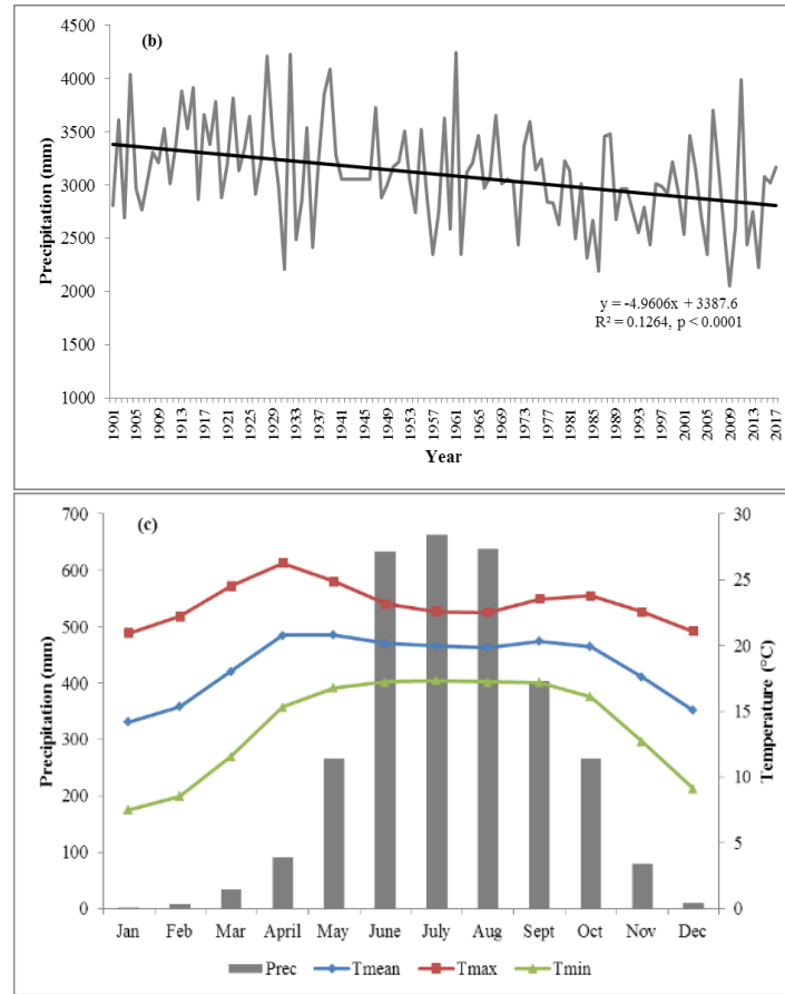
Figure 2. Annual precipitation and temperatures from 1901–2017 over the study area, Natma Taung National Park, Myanmar. Red line = maximum temperature, blue line = mean temperature, green line = minimum temperature, grey line and bar = precipitation. (a) Mean annual temperatures; (b) mean annual precipitation and (c) mean monthly precipitation and temperatures.
